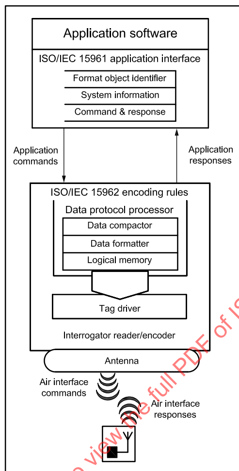
Figure 3 — ISO RFID data protocol architecture
