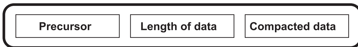
Figure 4 — ISO/IEC data set with Relative-OID values 1 to 14
