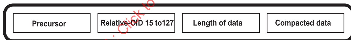
Figure 5 — ISO/IEC data set with Relative-OID values 15 to 127
