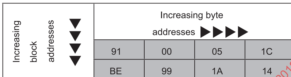
Figure 7 — Encoded bytes for example in Table D.3
