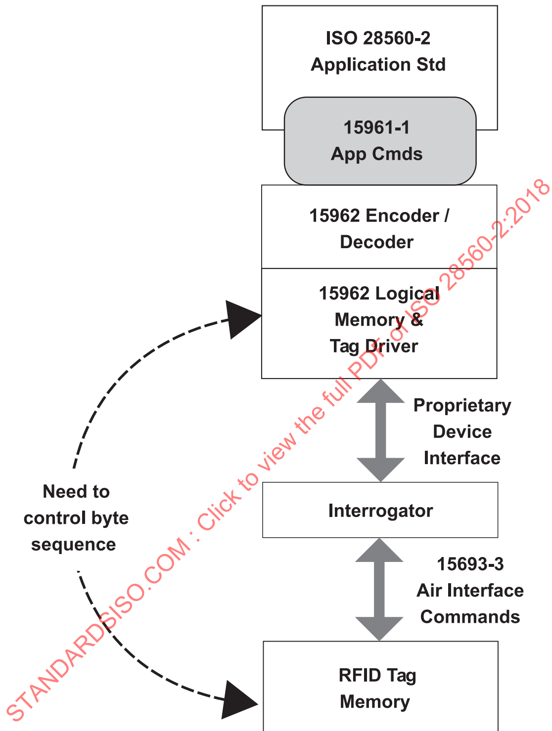
Figure 6 — Issues and constraints on bit and byte sequence
