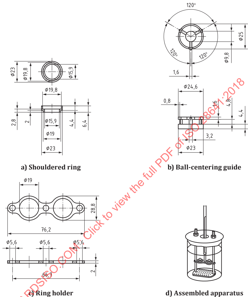
Figure 5 — Softening point measurement apparatus (example)
