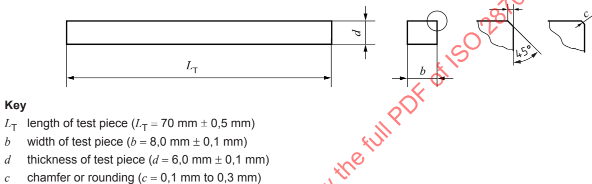
Figure 4 — Test piece dimensions and chamfering of ridge line
