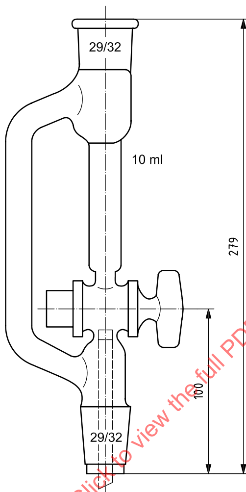
Figure 4 — Graduated collector
