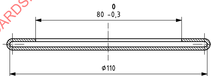
Figure 5 — Protective envelope
