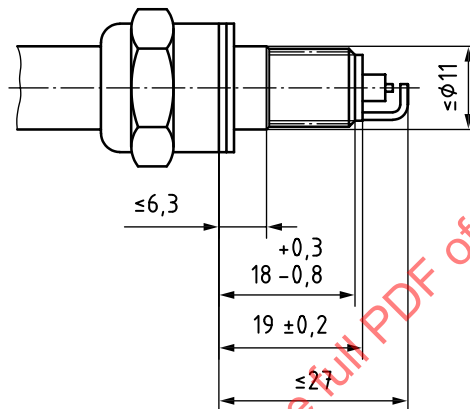
Figure A.1 — Spark plug with half thread
