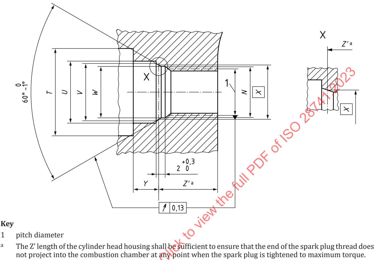
Figure 11 — Cylinder head housing for conical seating
