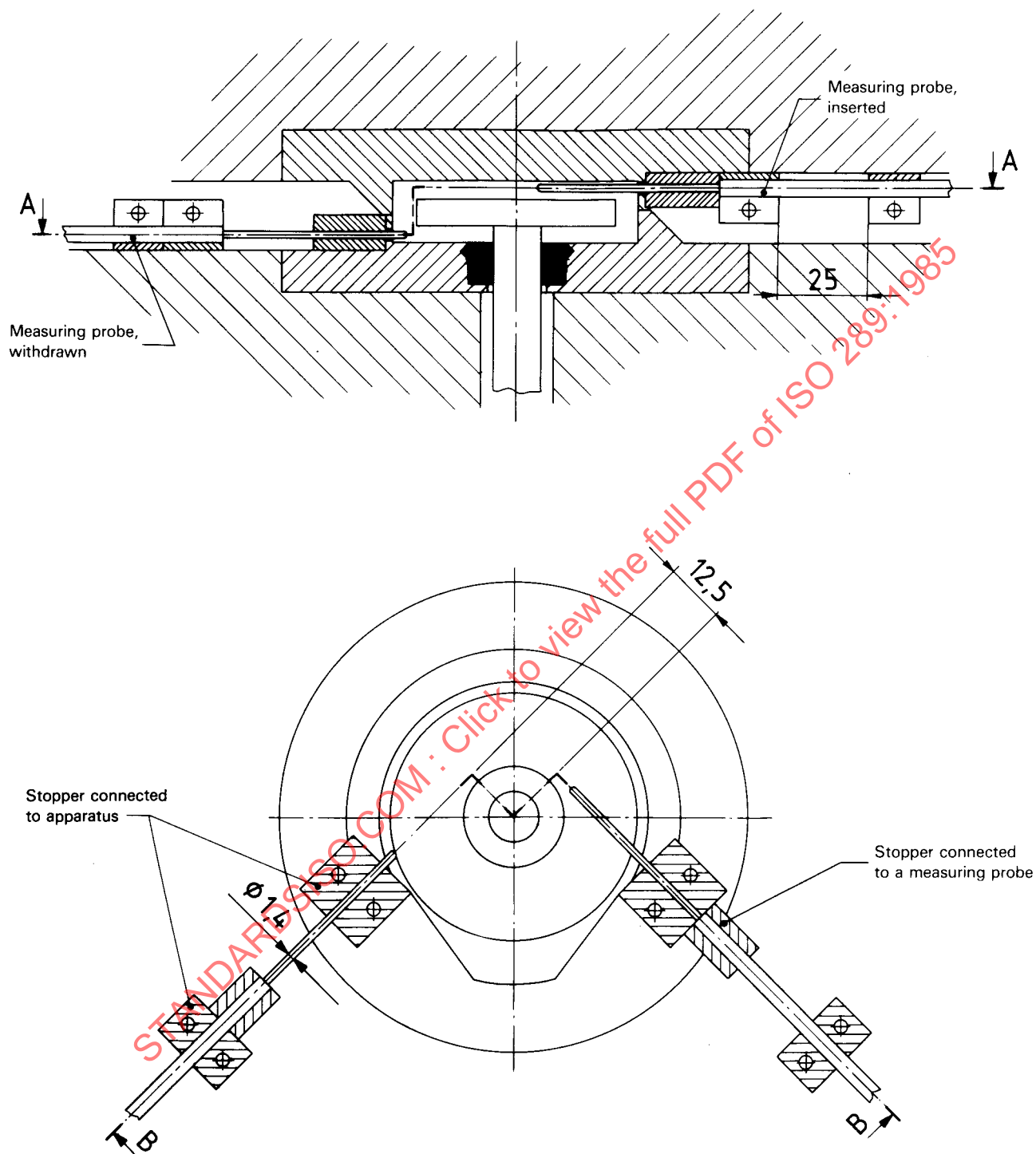
Figure 4 — Measuring probe design
