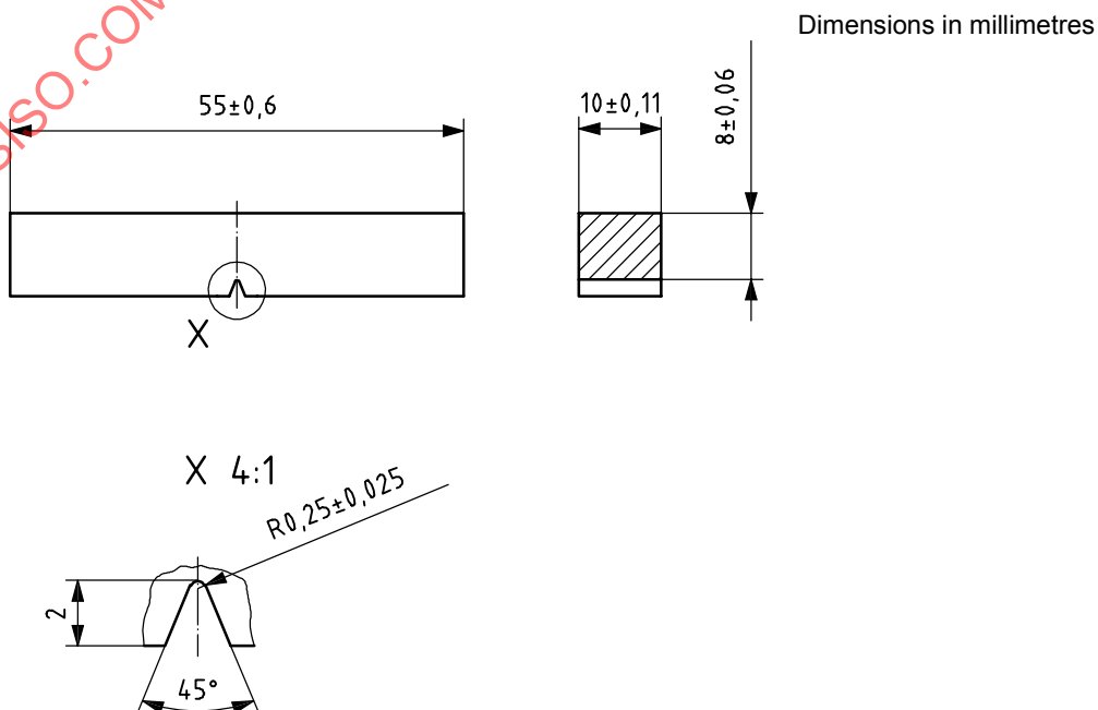
Figure 5 — Charpy V-notched impact test piece
