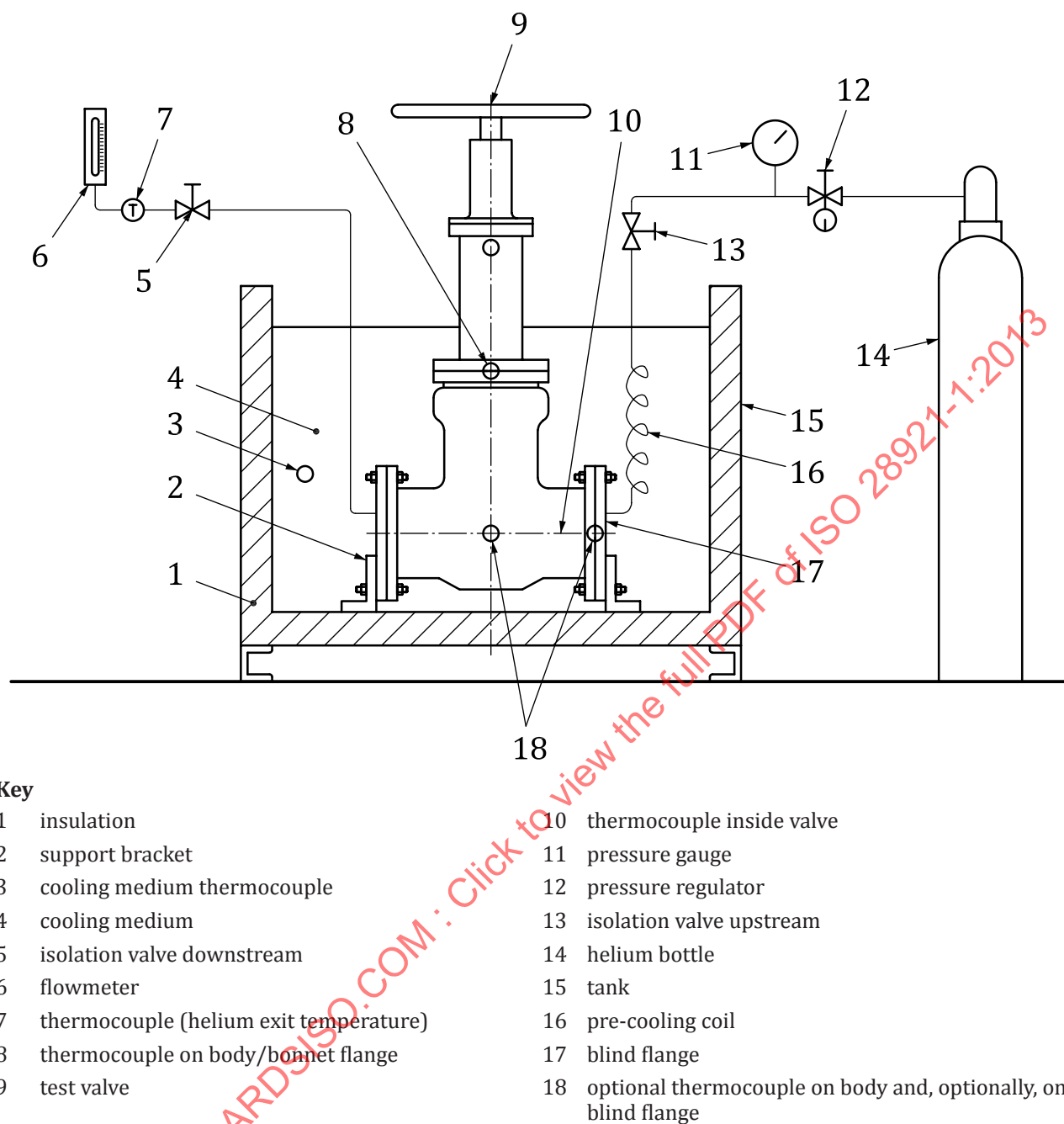
Figure A.2 — Test set-up
