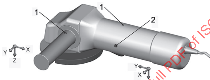
Figure 7 — Measurement locations — Electrical angle grinder with separate main handle
