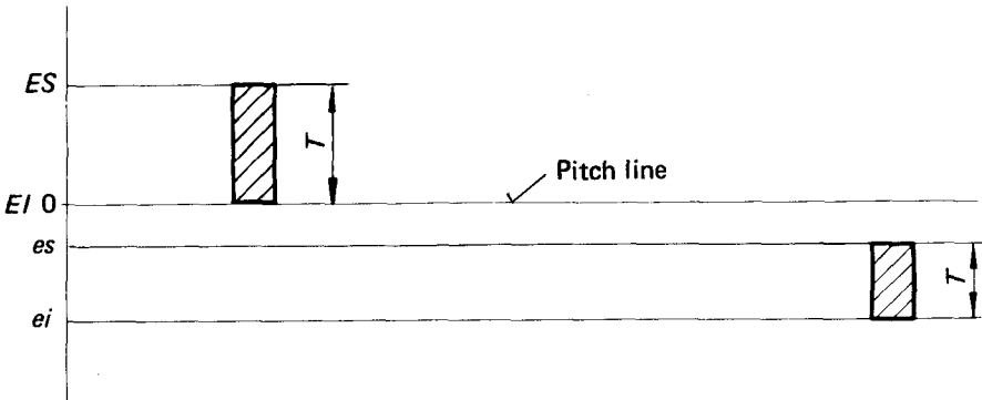
FIGURE 1 – Tolerance positions with respect to zero line (basic size)
