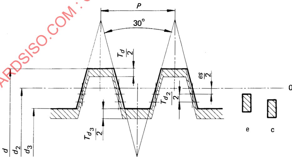
FIGURE 3 – Bolt threads with tolerance positions c and e for the pitch diameter
