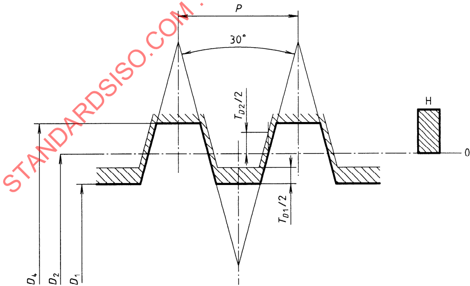
Figure 2 — Nut threads with tolerance position H for the pitch diameter
