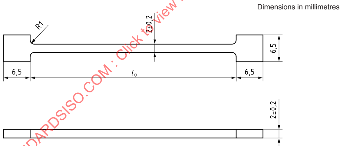
Figure 2 — Test piece
