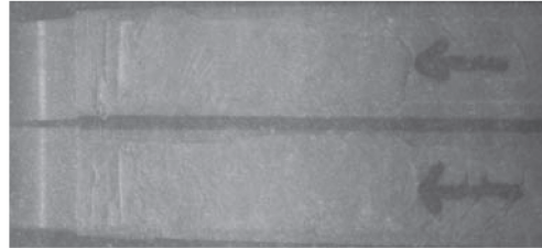
Figure 7 — Fracture surface of two halves of crack run-arrest specimen indicating the crack-arrest position
