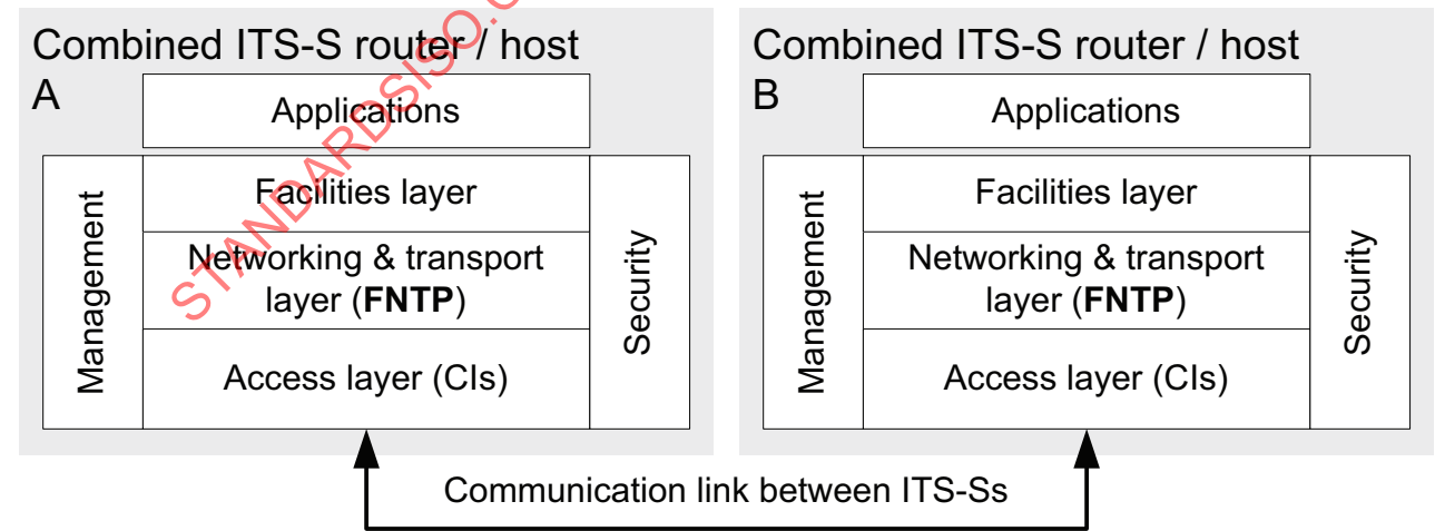
Figure 2 — Implementation architecture I
