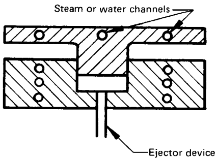
FIGURE 5 — Section of mould cored for steam heating and water cooling
