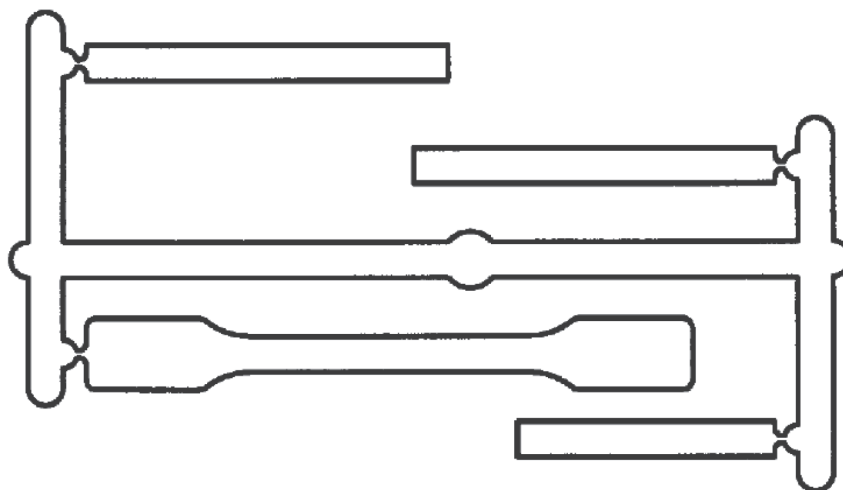
Figure 5 — Example of a family mould
