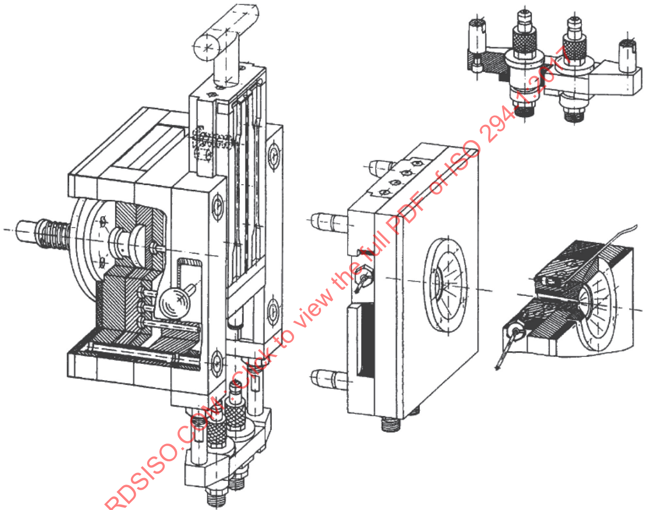
Figure C.1 — Exploded view of an injection mould with an interchangeable two-cavity plate for an ISO 20753 type A1 mould
