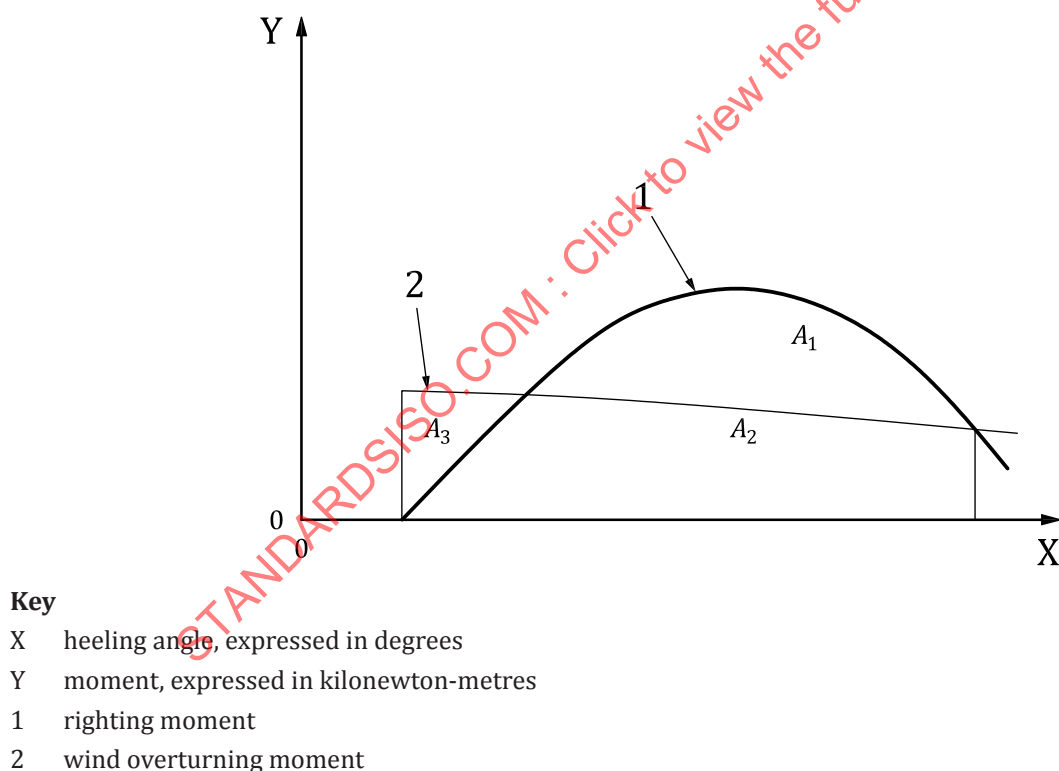
Figure 5 — Damage stability requirements for non-jack-up vessels [8]
