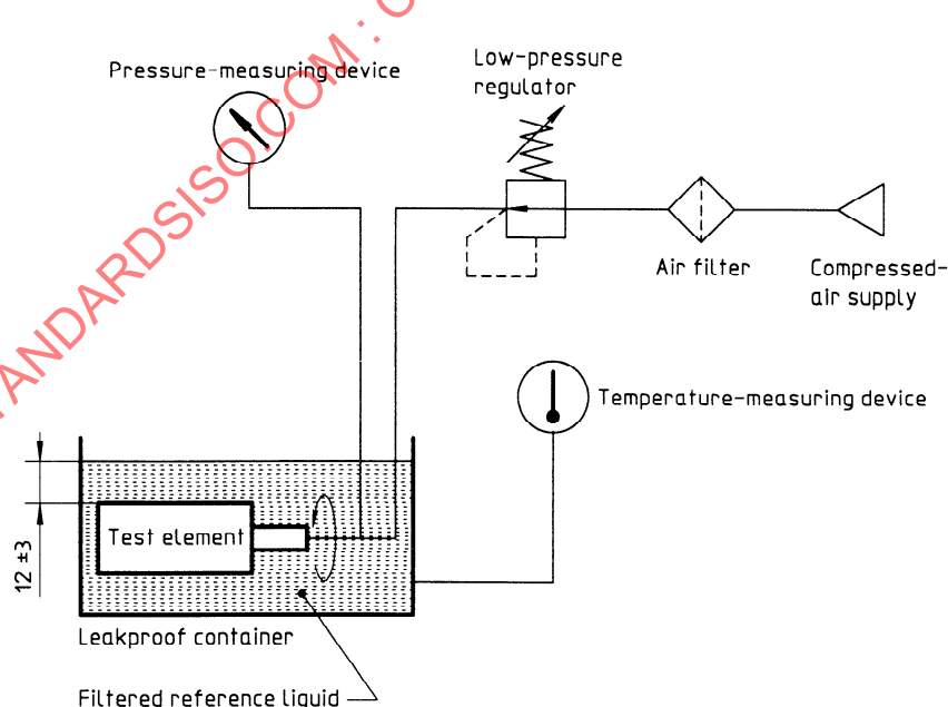
Figure 1 — Typical bubble-point testing apparatus
