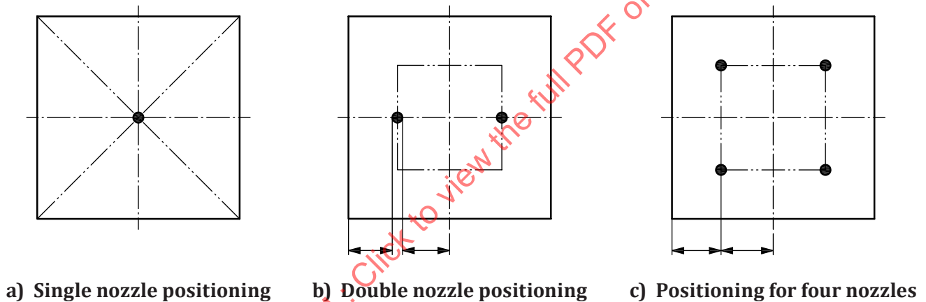
Figure 2 — Positioning of feeding nozzles
