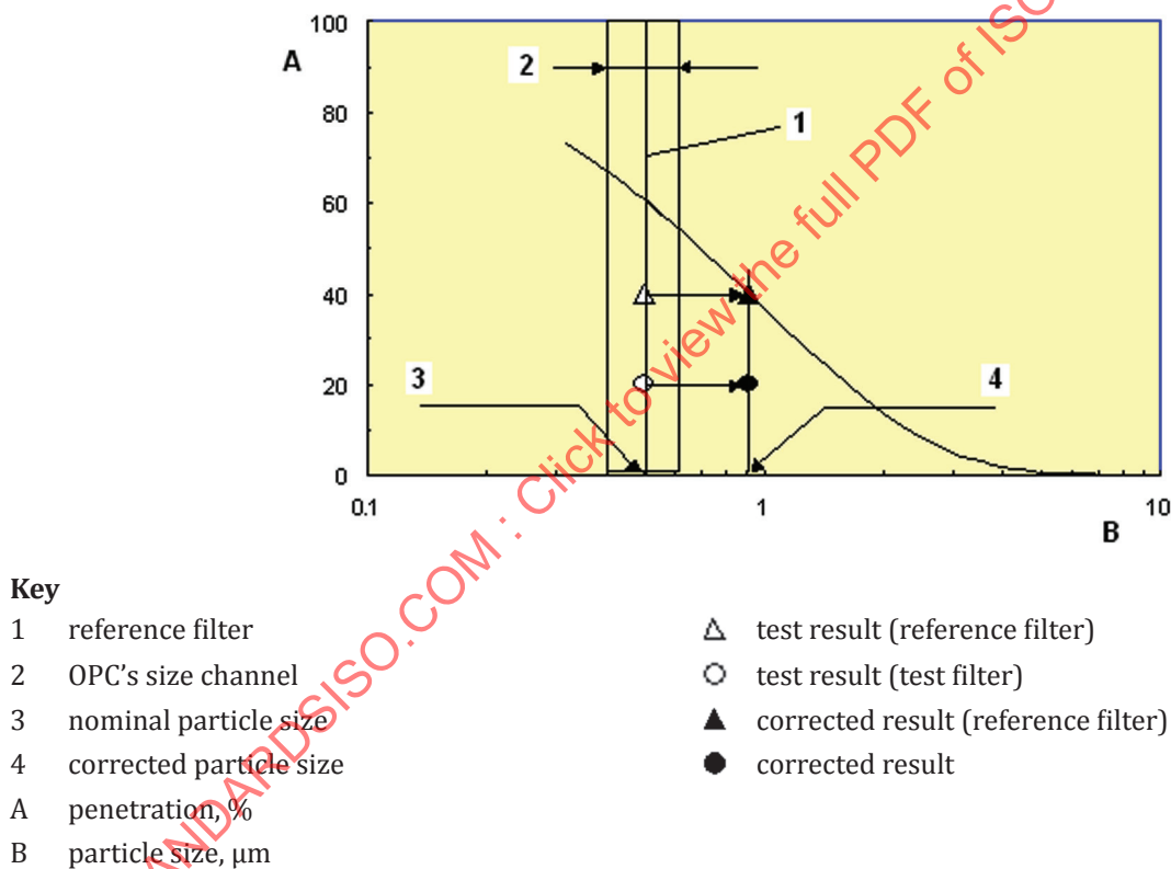
Figure 6 — Determination of the corrected particle size
