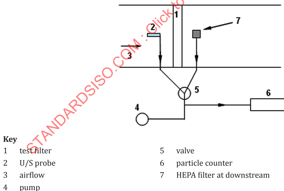
Figure 4 — Checking zero count at downstream sampling line
