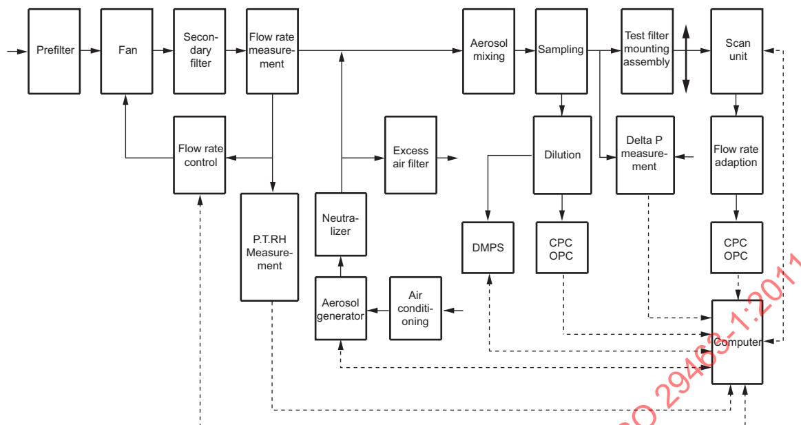
Figure 3 — Arrangement of apparatus for leak testing
