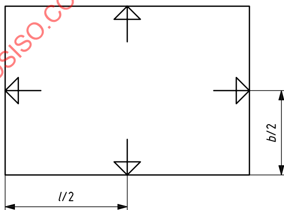
Figure 1 — Positions for measuring length and width of a test specimen where l \leq 1,5 \text{ m} and b \leq 1,5 \text{ m}
