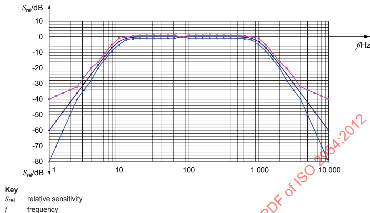
Figure 1 — Nominal values in decibels of relative sensitivity and limits of permissible deviations
