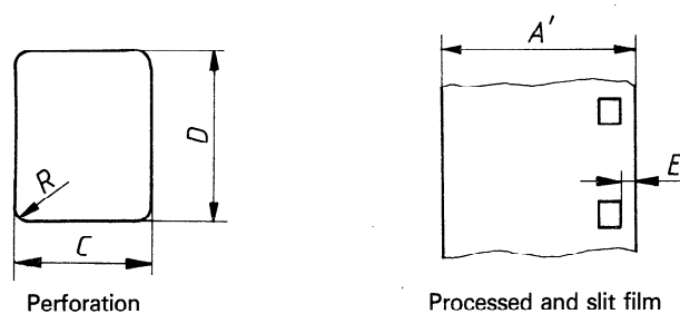
Figure 3 — Detail of perforation and width of processed and slit film
