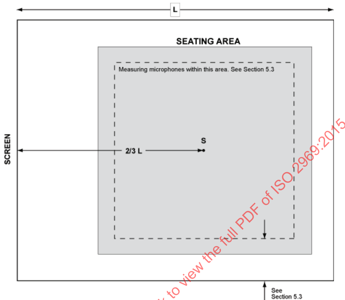
Figure 4 — Range of microphone placements
