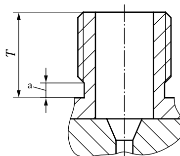
Figure 5 — Fabricated 60° female cone without undercut
