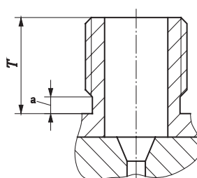
Figure 5 — Fabricated 60° female cone without undercut
