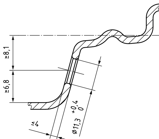
Figure 2 — Valve hole dimensions for snap-in valves
