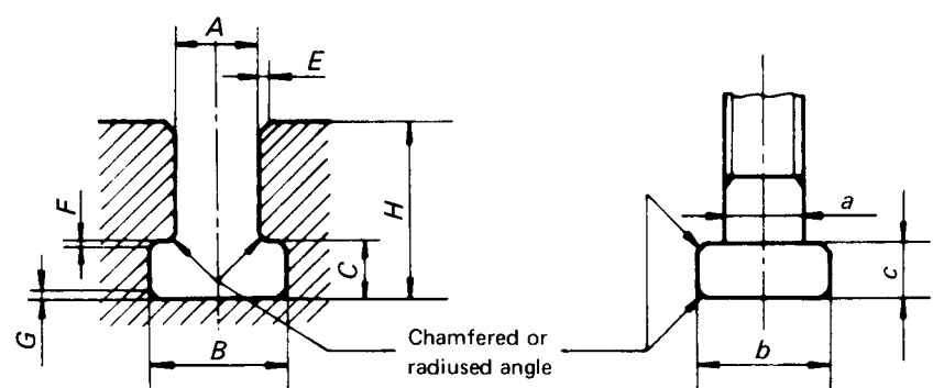
E, F and G : 45°-chamfer height or radius
