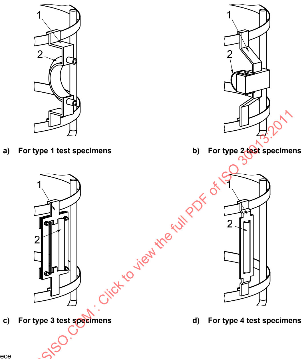
Figure 6 — Examples of clamps for attaching mandrels/test piece holders to the exposure frame
