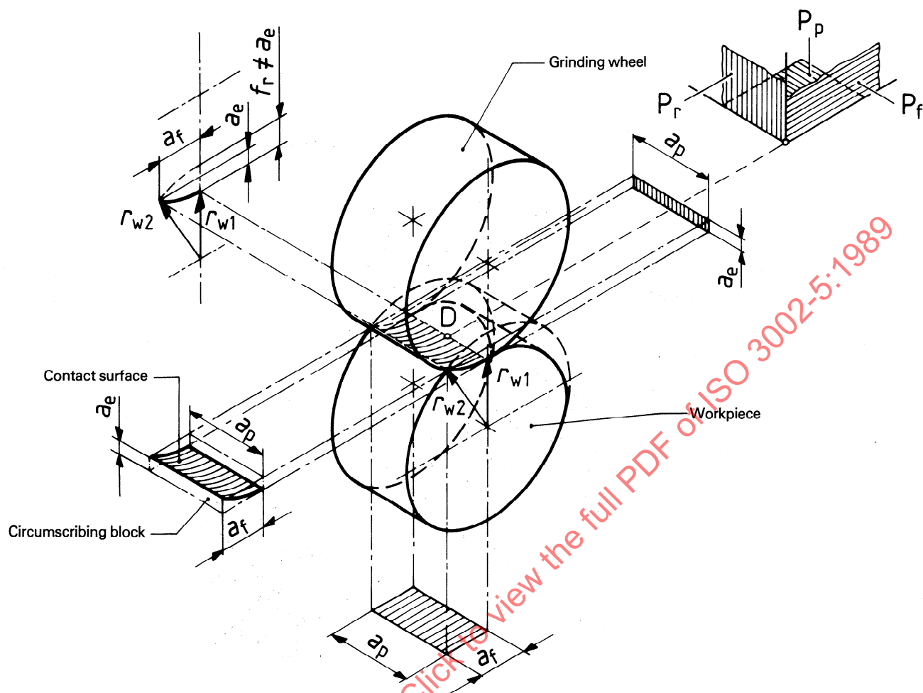
Figure 7 — Feed and engagement in peripheral grinding
