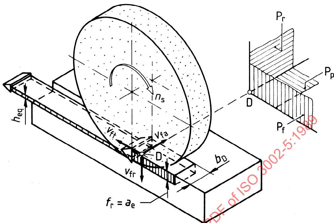
Figure 3 — Equivalent grinding thickness, motions and reference system of planes in surface, peripheral and tangential grinding
