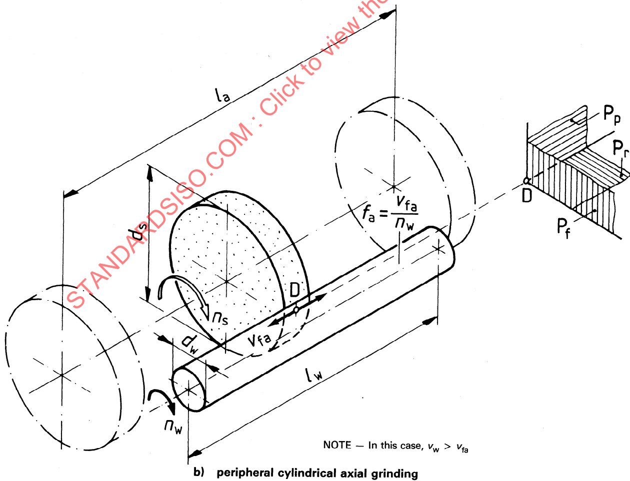
Figure 2 — Motions and reference system of planes in peripheral cylindrical grinding
