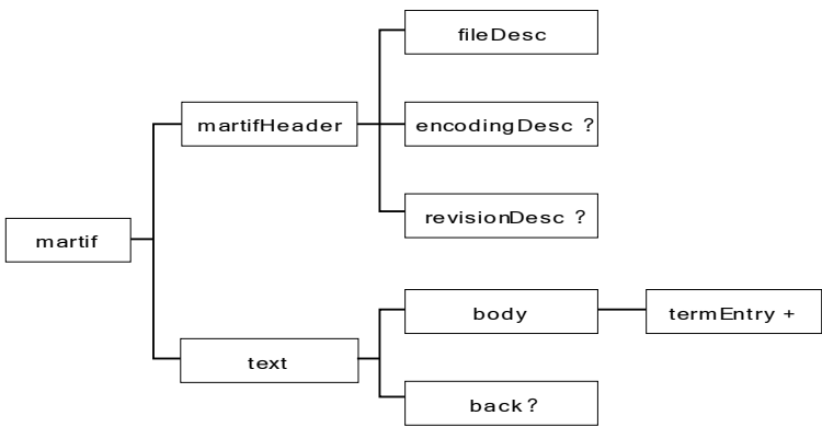
Figure 2. The MARTIF structure
