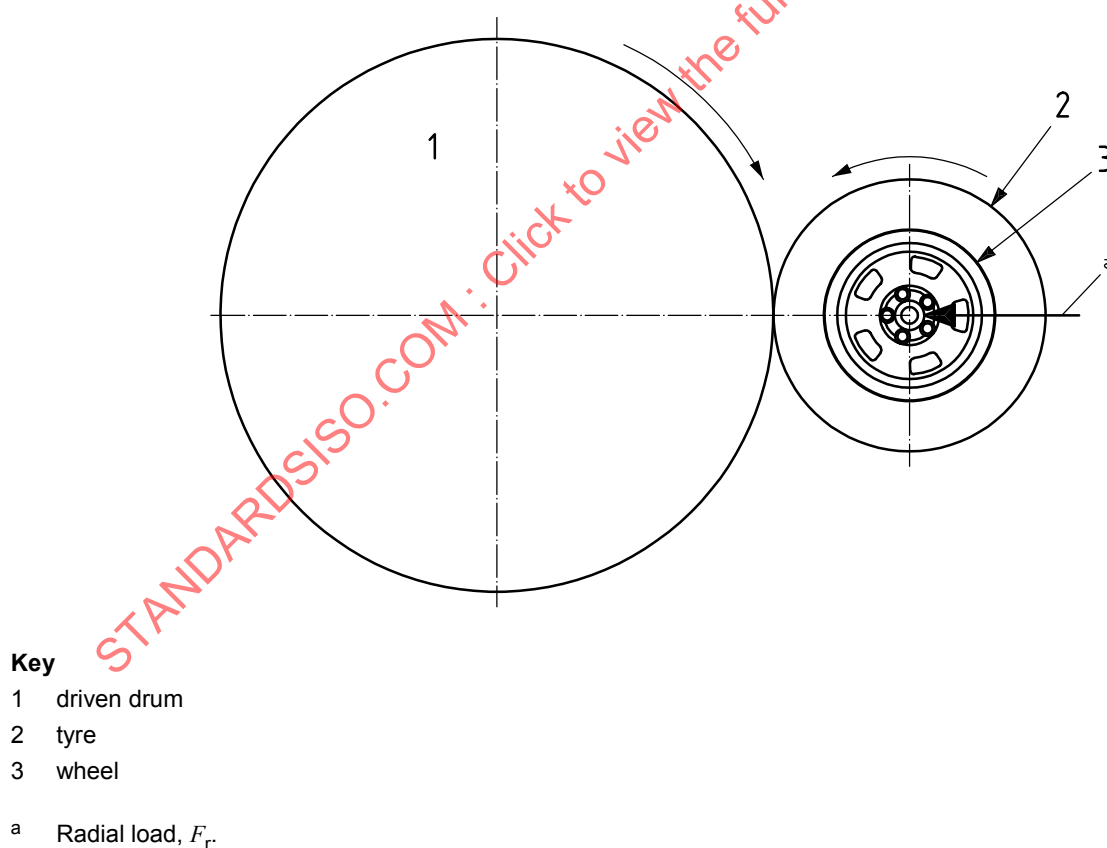
Figure 2 — Example of dynamic radial fatigue test fixture
