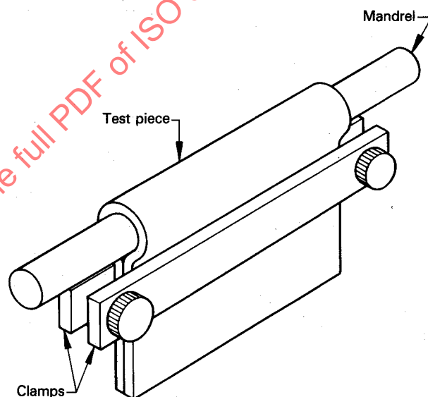
Figure — Test piece holder
