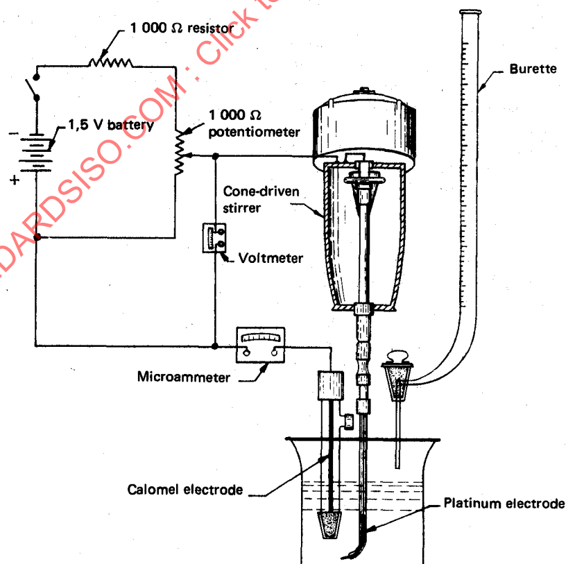
FIGURE 1 — Diagram of amperometric titration apparatus
