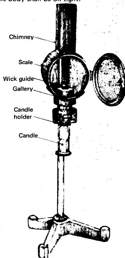
FIGURE 1 – Smoke point lamp
