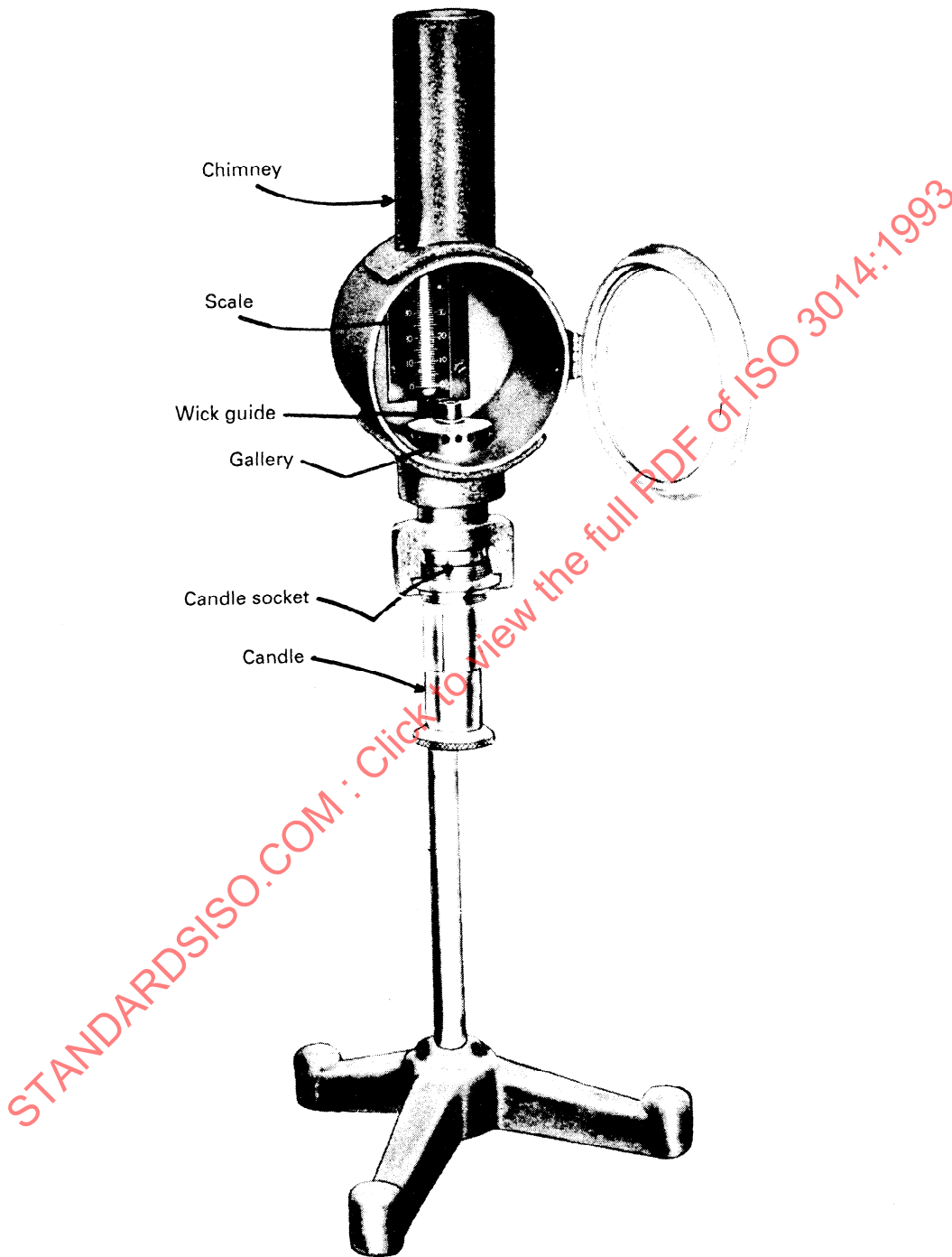
Figure 1 — Smoke-point lamp
