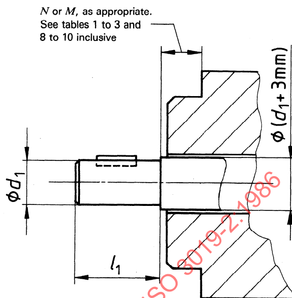
Figure 4 — Cylindrical shaft end with key
