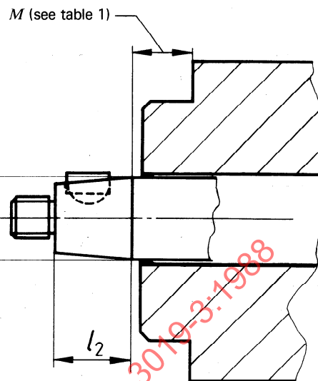
Figure 3 — Conical shaft end with key and external thread
