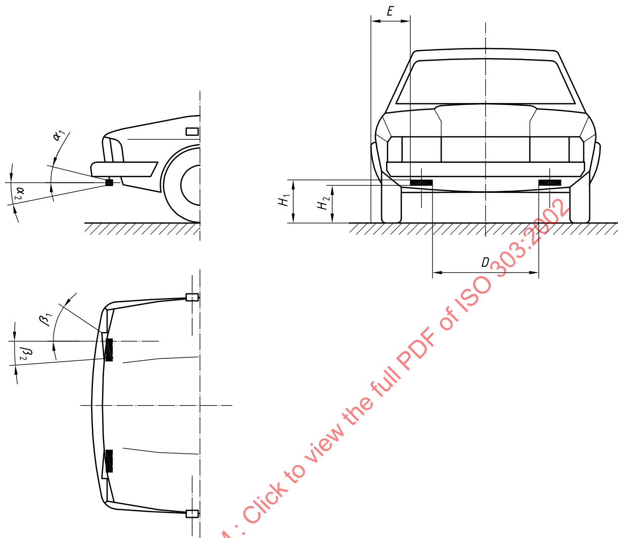
Figure E.4 — Front fog lamp
