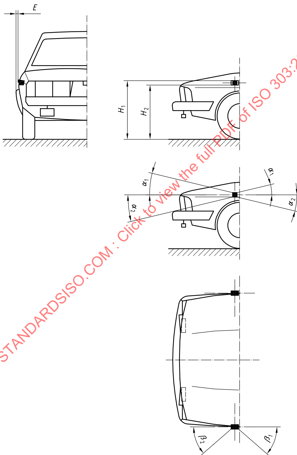
Figure E.6 — Parking lamp
