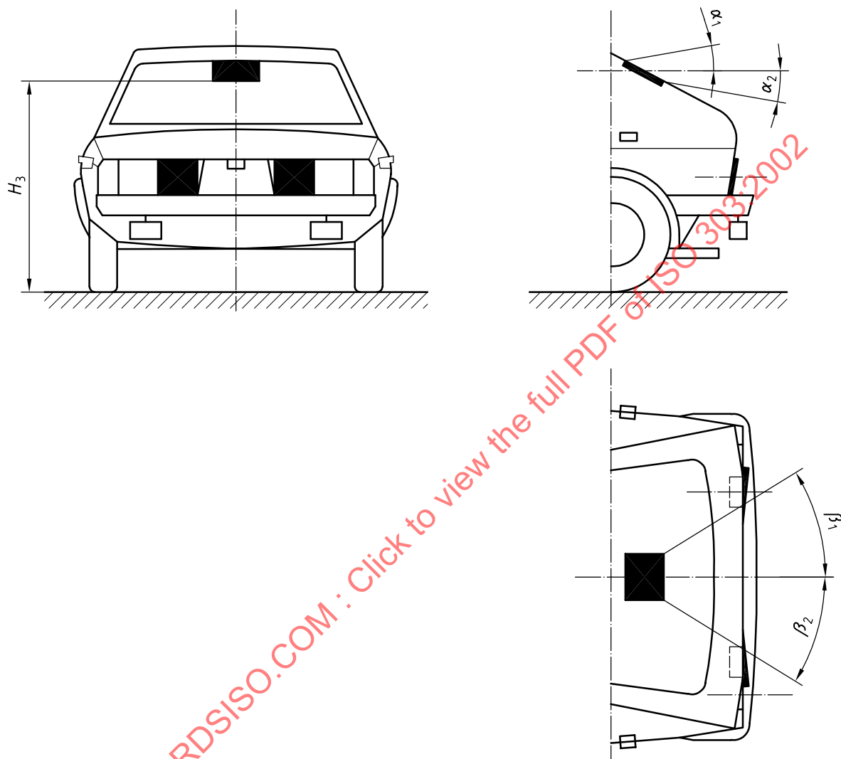
Figure E.11 — Stop lamp (centre high-mounted)
