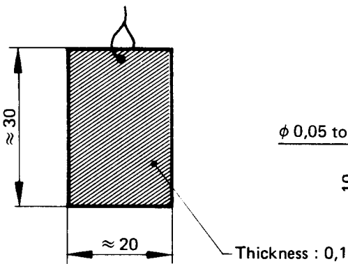
FIGURE 1 – Plate [5.2 a)]
