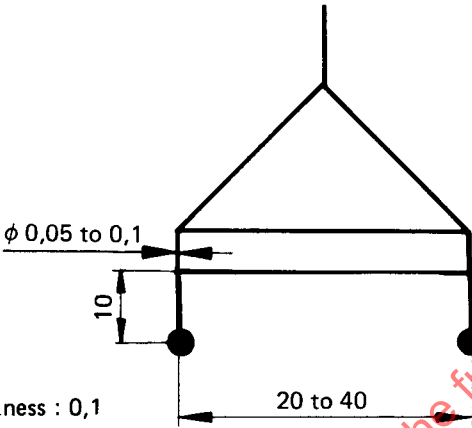
FIGURE 2 – Stirrup [5.2 b)]
