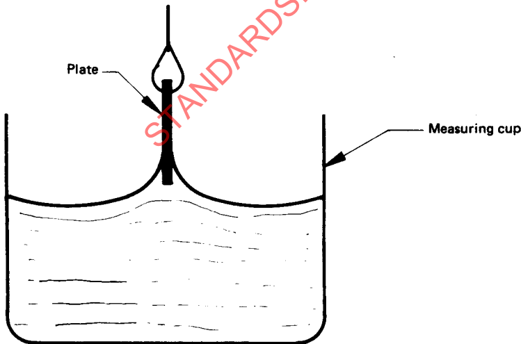
FIGURE 4 – Measurement using a plate
