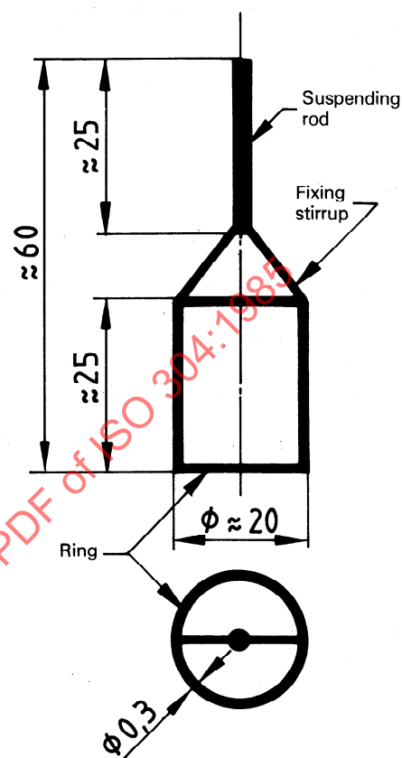
Figure 3 — Ring [5.2 c)]
