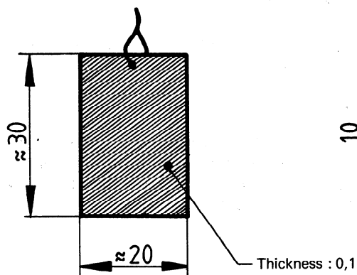
Figure 1 — Plate [5.2 a)]
