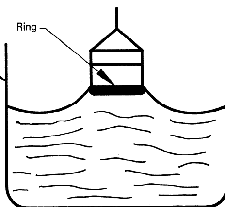
Figure 5 — Measurement using a ring
