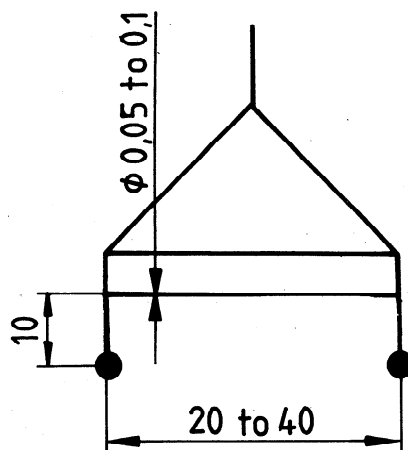
Figure 2 — Stirrup [5.2 b)]
