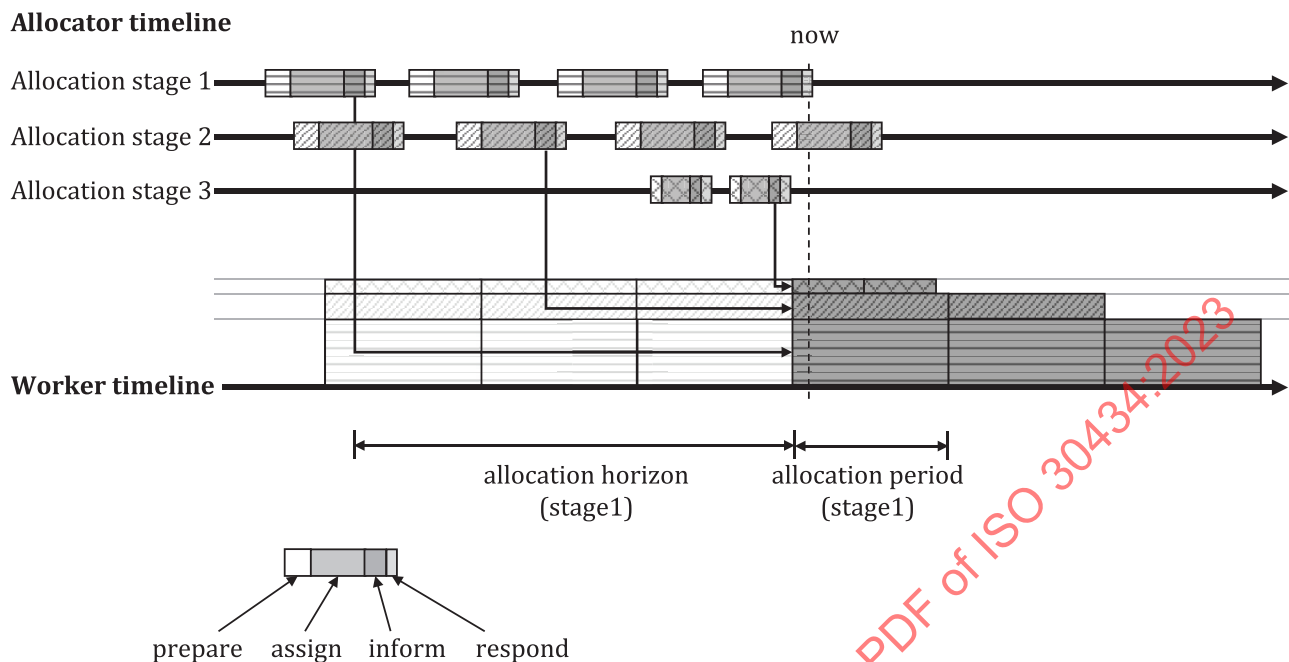
Figure 3 — Allocation stages, steps, horizon and period
