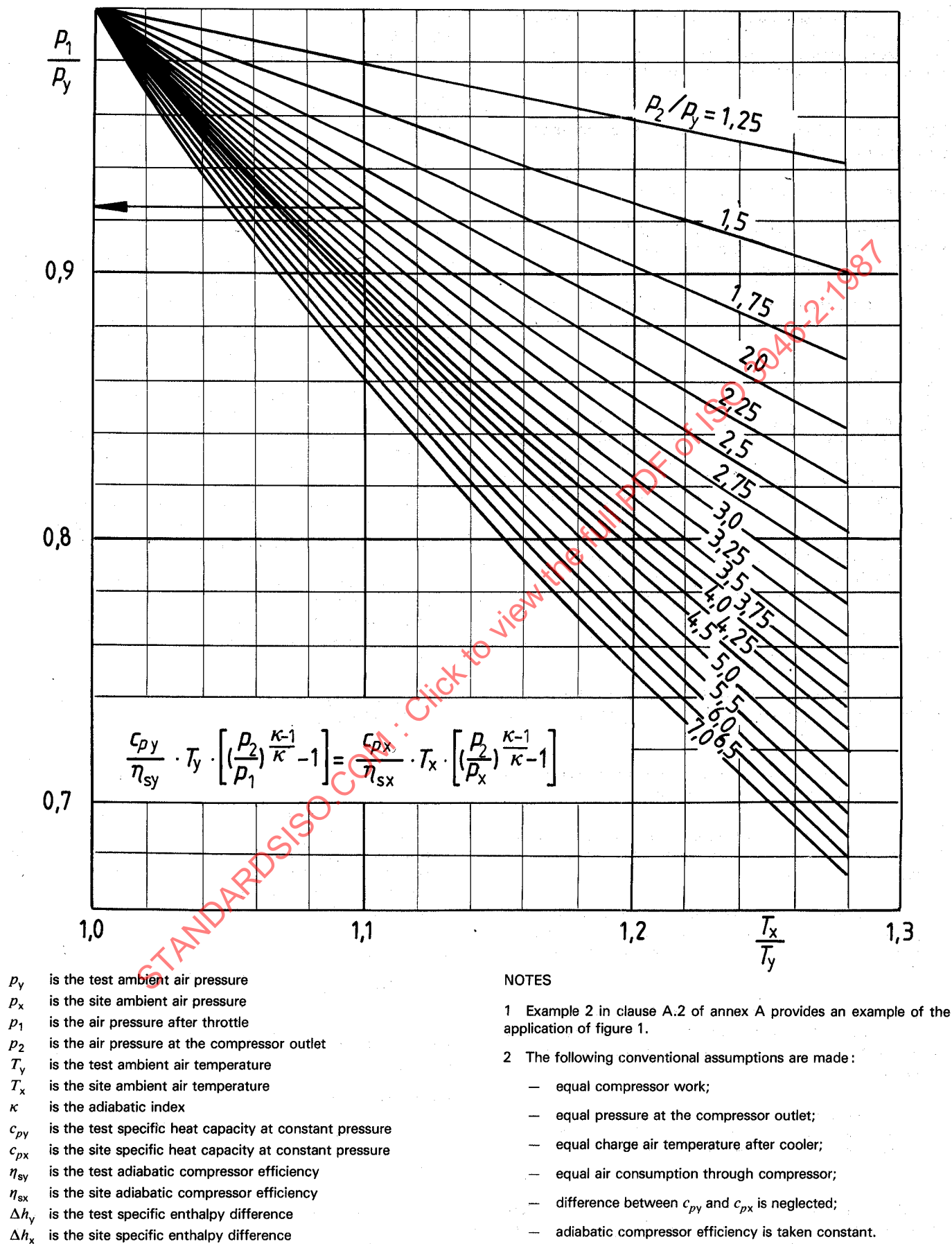
Figure 1 — Determination of depression at compressor inlet when simulating high on-site air temperature
