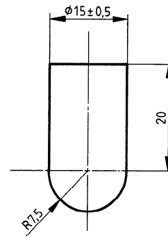
Figure 1 — Aluminium block
