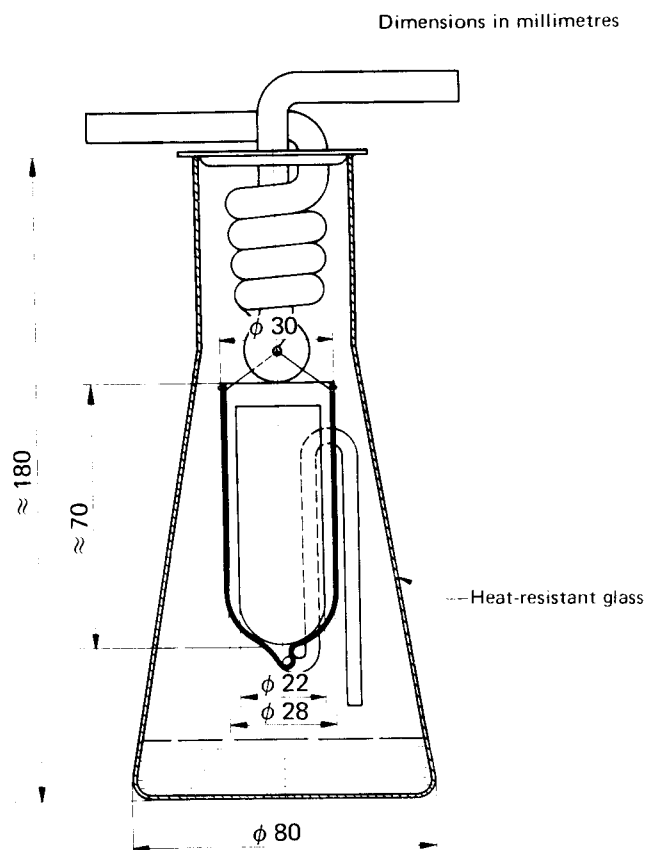
FIGURE — Extraction apparatus
