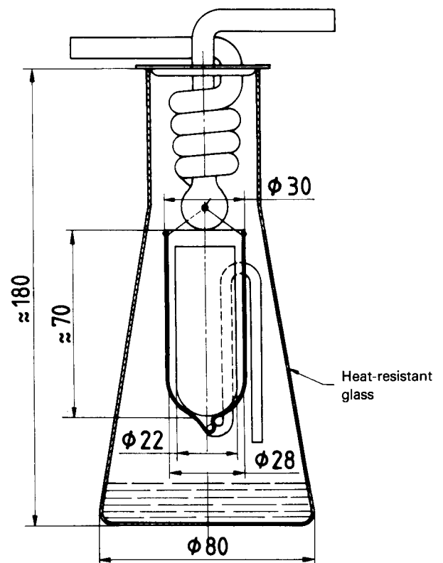
Figure — Extraction apparatus
