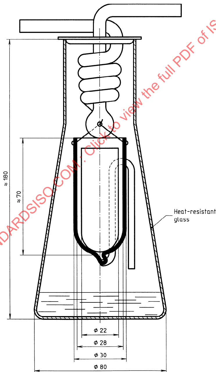
Figure 1 — Extraction apparatus
