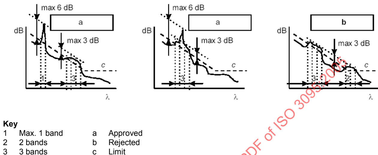
Figure A.4 — Examples of application of the rail roughness spectrum approval criterion
